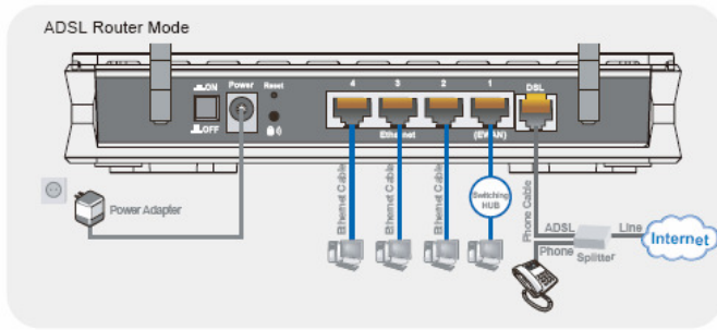
ADSL Router Mode
