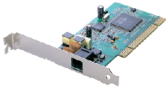
▲ BIPAC-702AE
